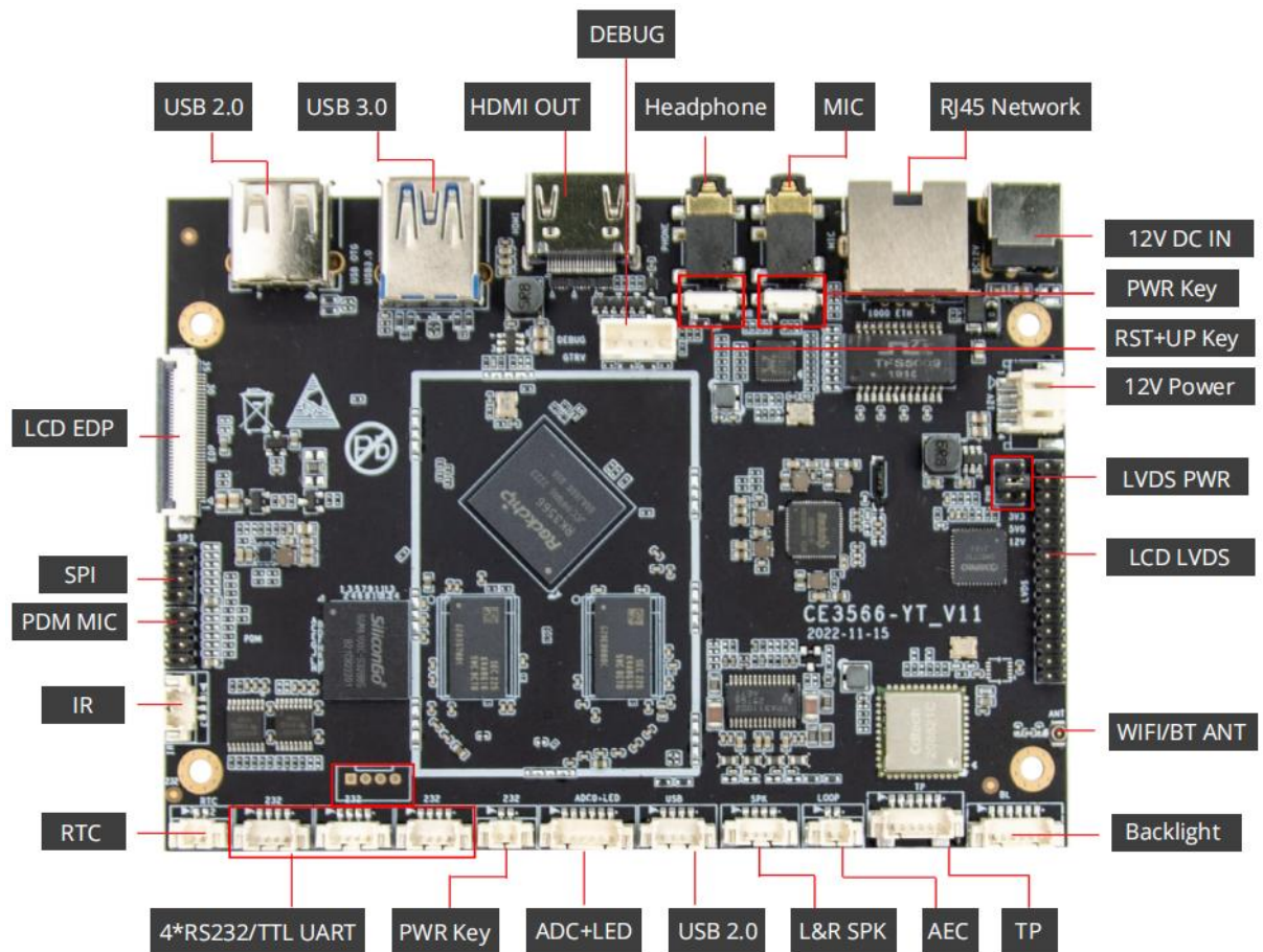
Figure 2 Front View of the DEBIX R3566-01
